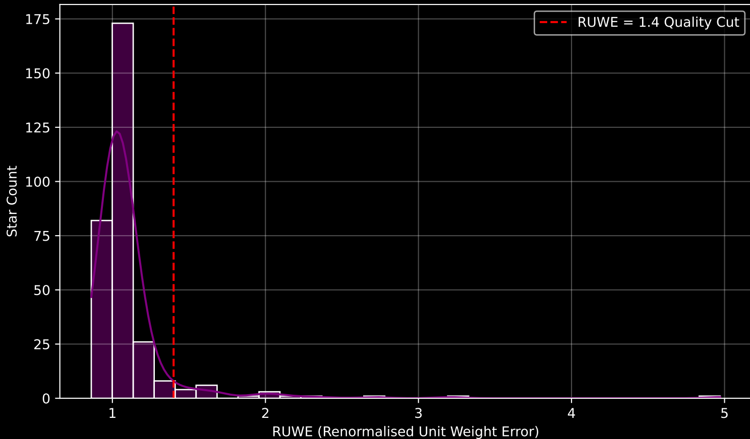
GAPOGEE DR17 Field [160+12] RUWE Distribution (n= 308)
