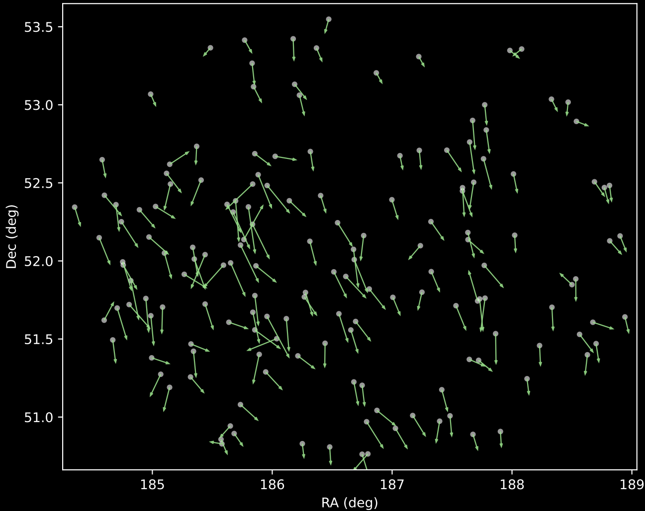
APOGEE DR17 Cluster 5 Proper Motion Vectors (n=159)
