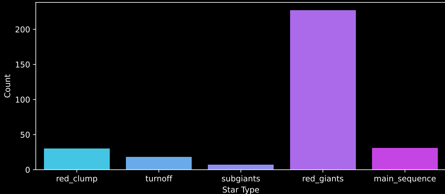
APOGEE DR17 Field: [160+12] Count plot of Star Type
