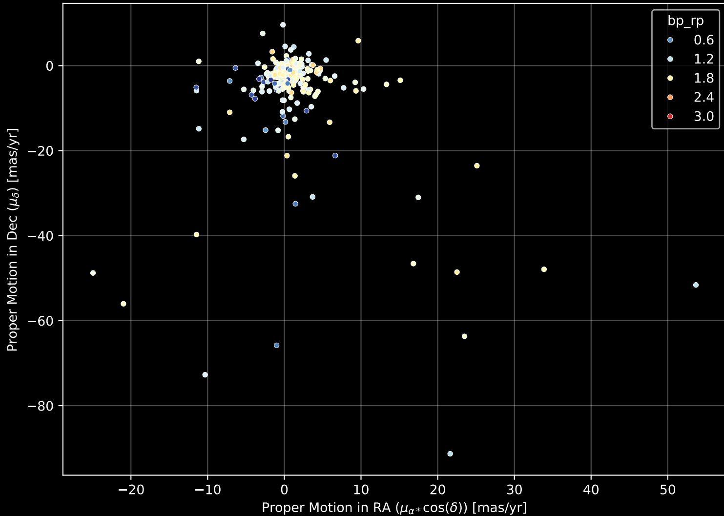
APOGEE DR17 Field: [160+12] Proper Motion Diagram (n= 313)
