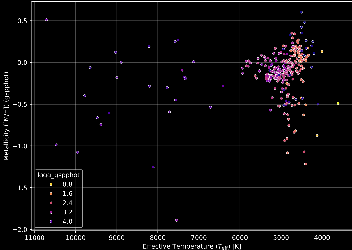
APOGEE DR17 Field: [160+12] Stellar Population Parameters (n= 313)
