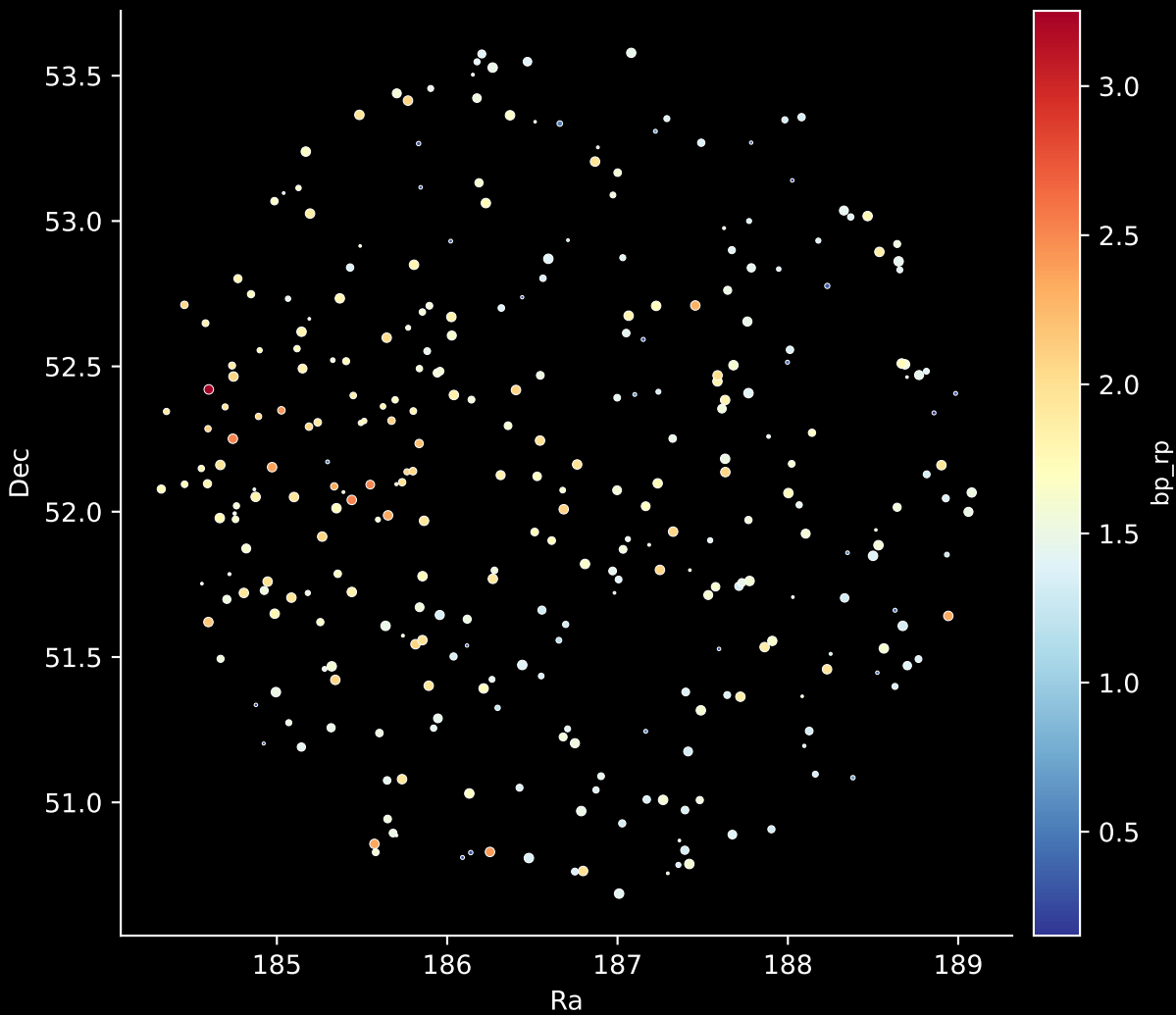
APOGEE DR17 Field: [160+12] Stars: 313
