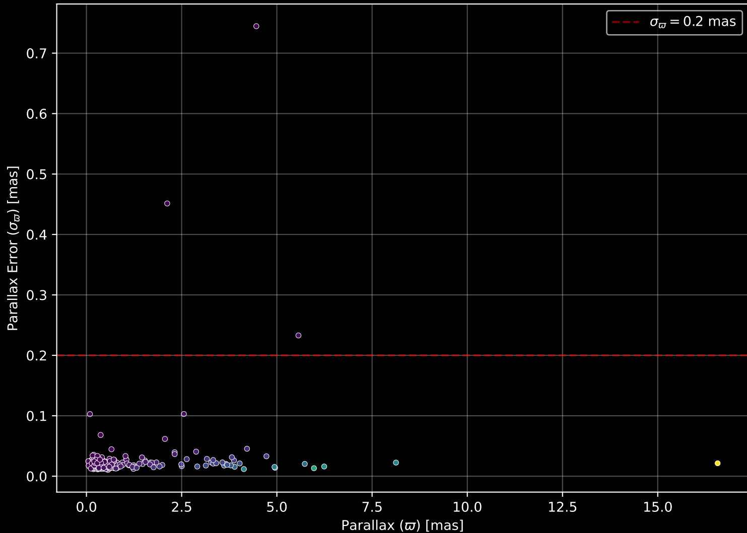
APOGEE DR17 Field: [160+12] Parallax Quality (n= 313)
