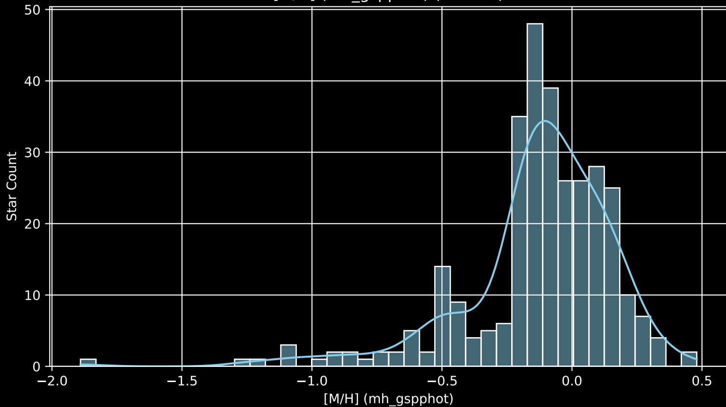
APOGEE DR17 Field: [160+12 [M/H] (mh_gspphot) (n= 311)
